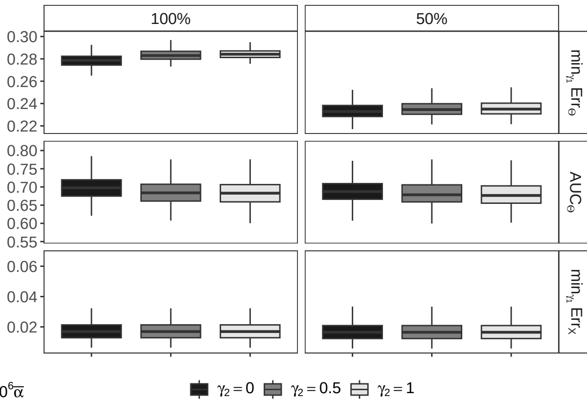
Banded graph structure
